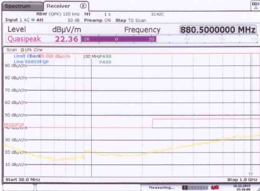
Antenna horizontal
