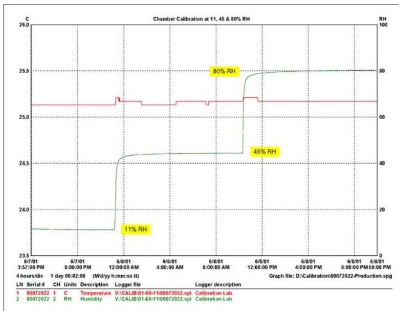
A typical 3-point data logger calibration cycle.
